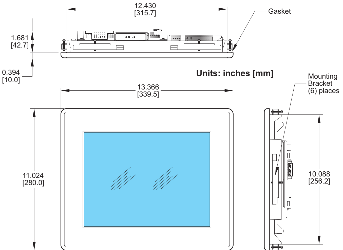
C-more 12" panel front and side view
